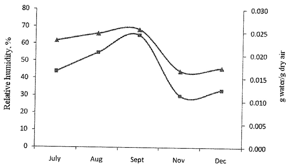
FIGURE 3. Relationship between actual amount of water in dry air (g water/g dry air) (■) and the measured relative humidity value (▲) in hot and humid condition.
