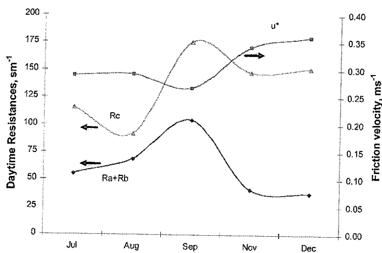
FIGURE 5. Monthly average aerodynamic resistance R_a and boundary layer resistance, R_b and canopy resistance at daytime
