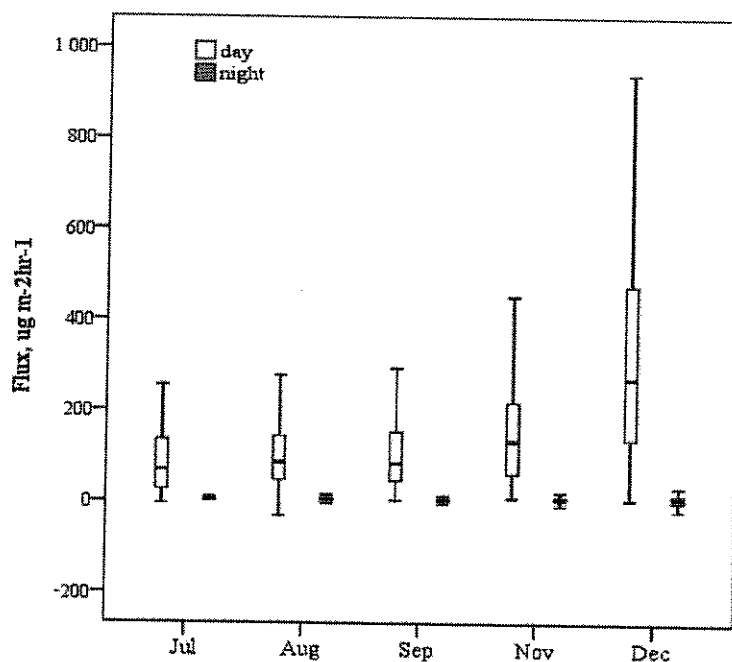
FIGURE 2. Effect of seasonal variation on SO 2 flux (July-September: wet season, November-December: dry season) in daytime, 8:00 - 17:00 hr and nighttime, 18:00 - 7:00 hr. The upper box is 75 percentile and the lower box is 25 percentile. The end of the spikes represent the maximum and the minimum values. The cross line in the box is the median value. 50% of data contained in the box
