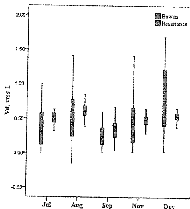
FIGURE 6. Median and percentiles of SO 2 deposition velocity calculated by the Bowen ratio method and the resistance model in daytime. The upper box is 75 percentile and the lower box is 25 percentile. The end of the spikes represent the maximum and the minimum values. The cross line in the box is the median value. 50% of data contained in the box
